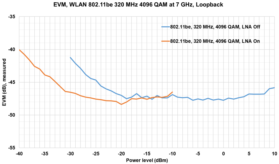
Figure 6. WLAN 802.11be EVM vs. output power level at 7 GHz, loopback
