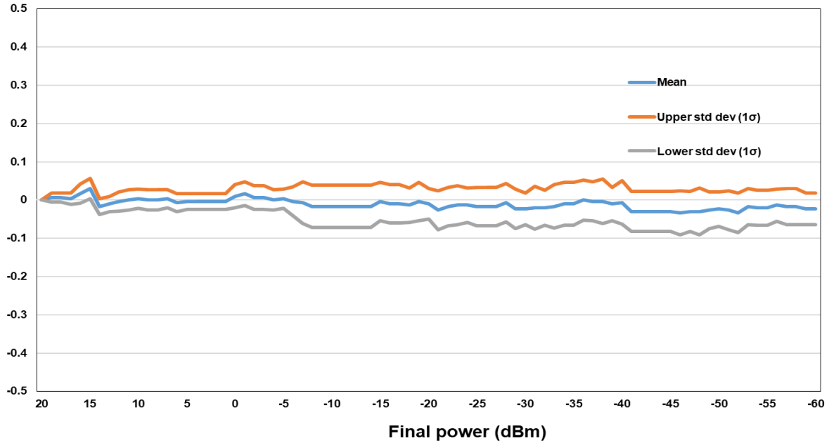
Measured relative level accuracy at 1 GHz initial power +20 dBm, 1 dB step
