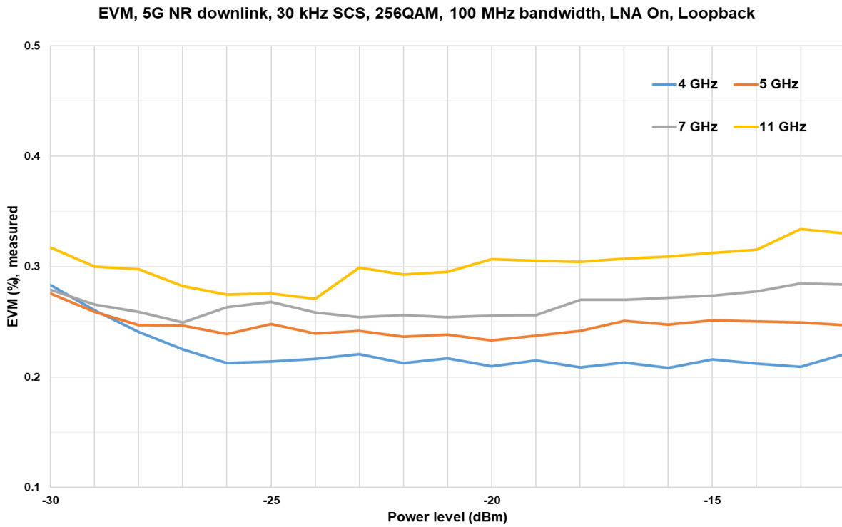
Figure 10. 5G NR downlink EVM vs. power level, LNA on, loopback, with 100 MHz bandwidth, 30 kHz SCS, 256QAM
