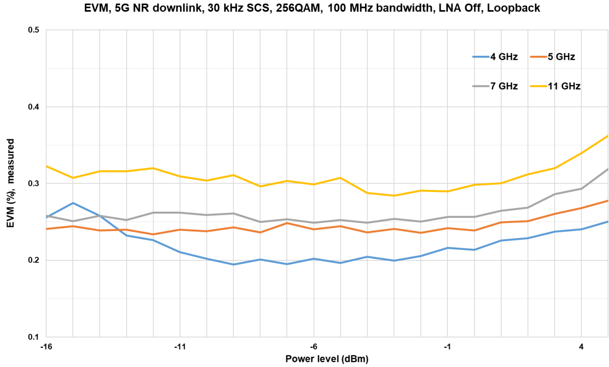
Figure 9. 5G NR downlink EVM vs. power level, LNA off, loopback, with 100 MHz bandwidth, 30 kHz SCS, 256QAM
