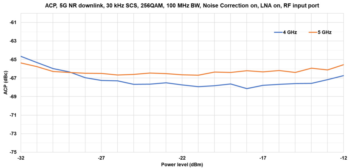
Figure 7. 5G NR downlink ACP vs. input power level, noise correction on, LNA on, 100 MHz bandwidth, 30 kHz SCS, 256QAM
